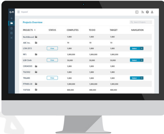
Q-FI Software
